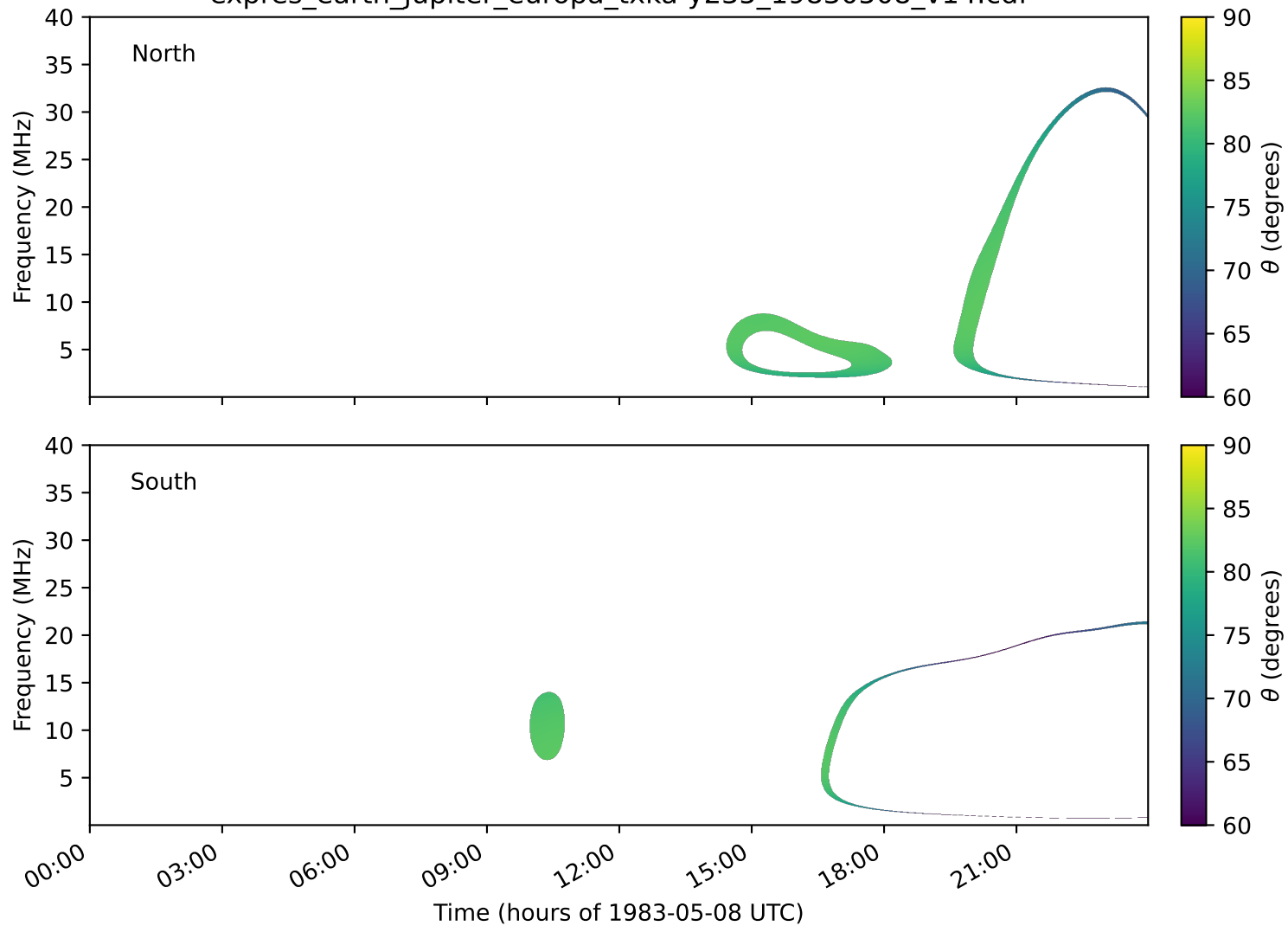
expres_earth_jupiter_europa_txka-y235_19830508_v14.cdf
