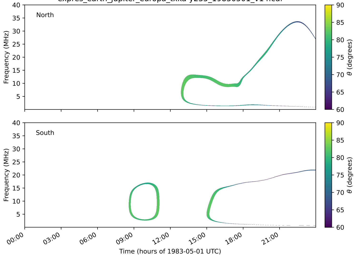
expres_earth_jupiter_europa_txka-y235_19830501_v14.cdf
