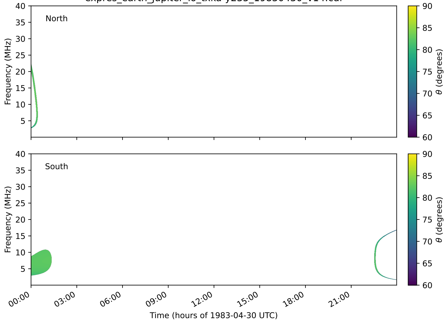
expres_earth_jupiter_io_txka-y235_19830430_v14.cdf
