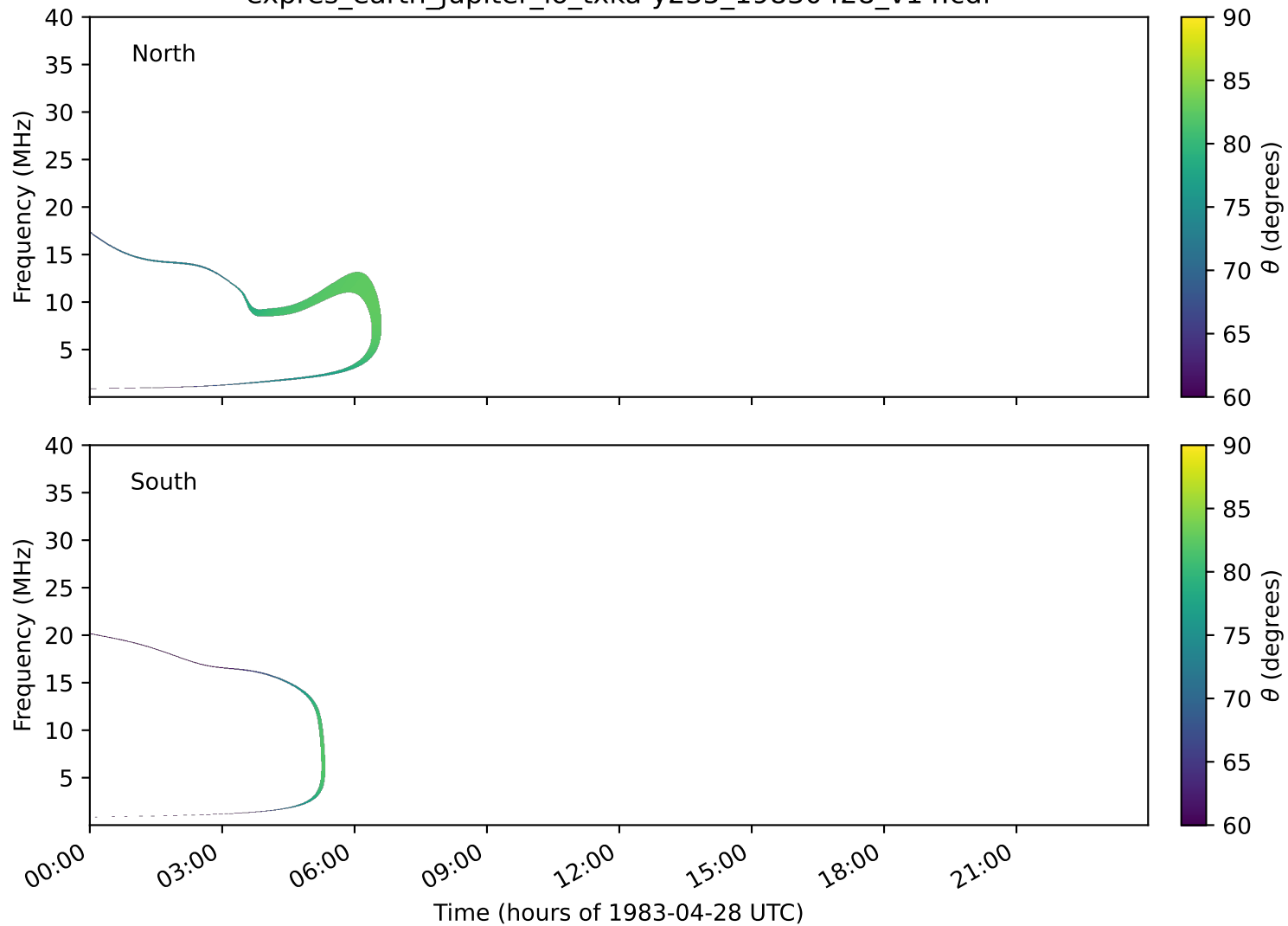
expres_earth_jupiter_io_txka-y235_19830428_v14.cdf
