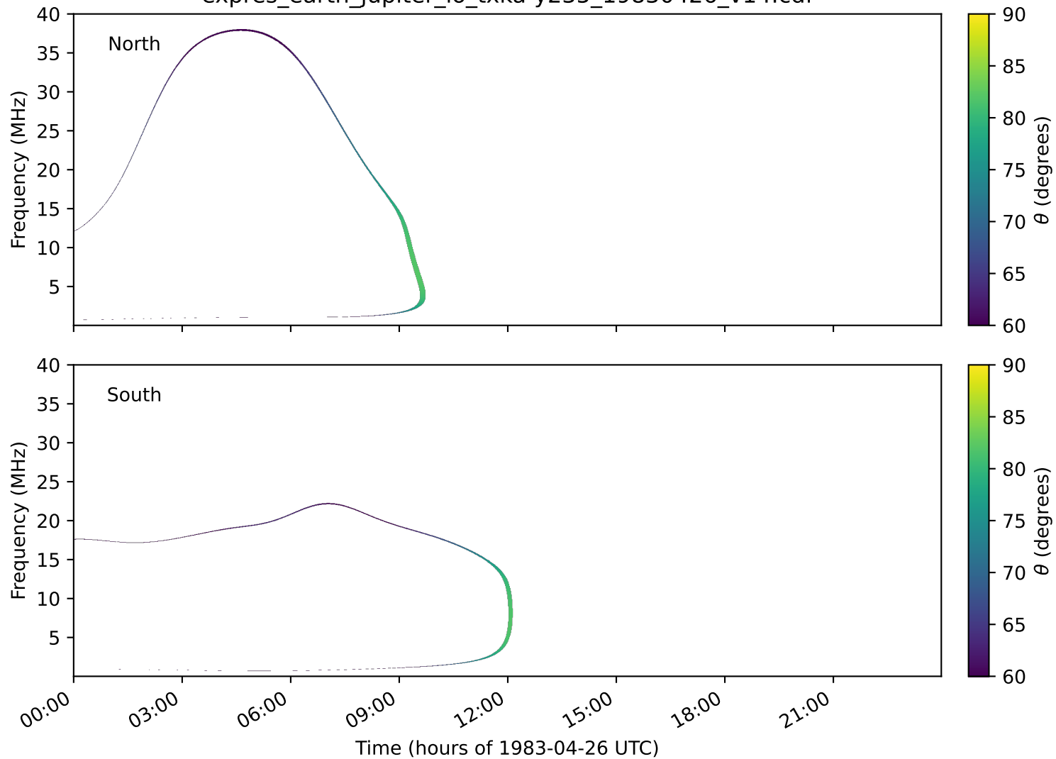
expres_earth_jupiter_io_txka-y235_19830426_v14.cdf
