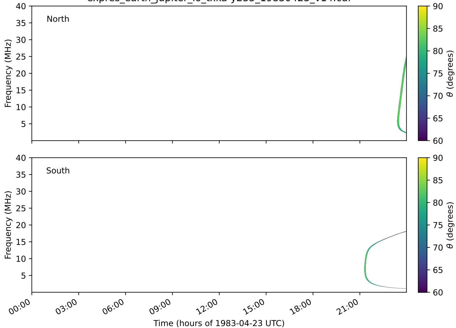
expres_earth_jupiter_io_txka-y235_19830423_v14.cdf
