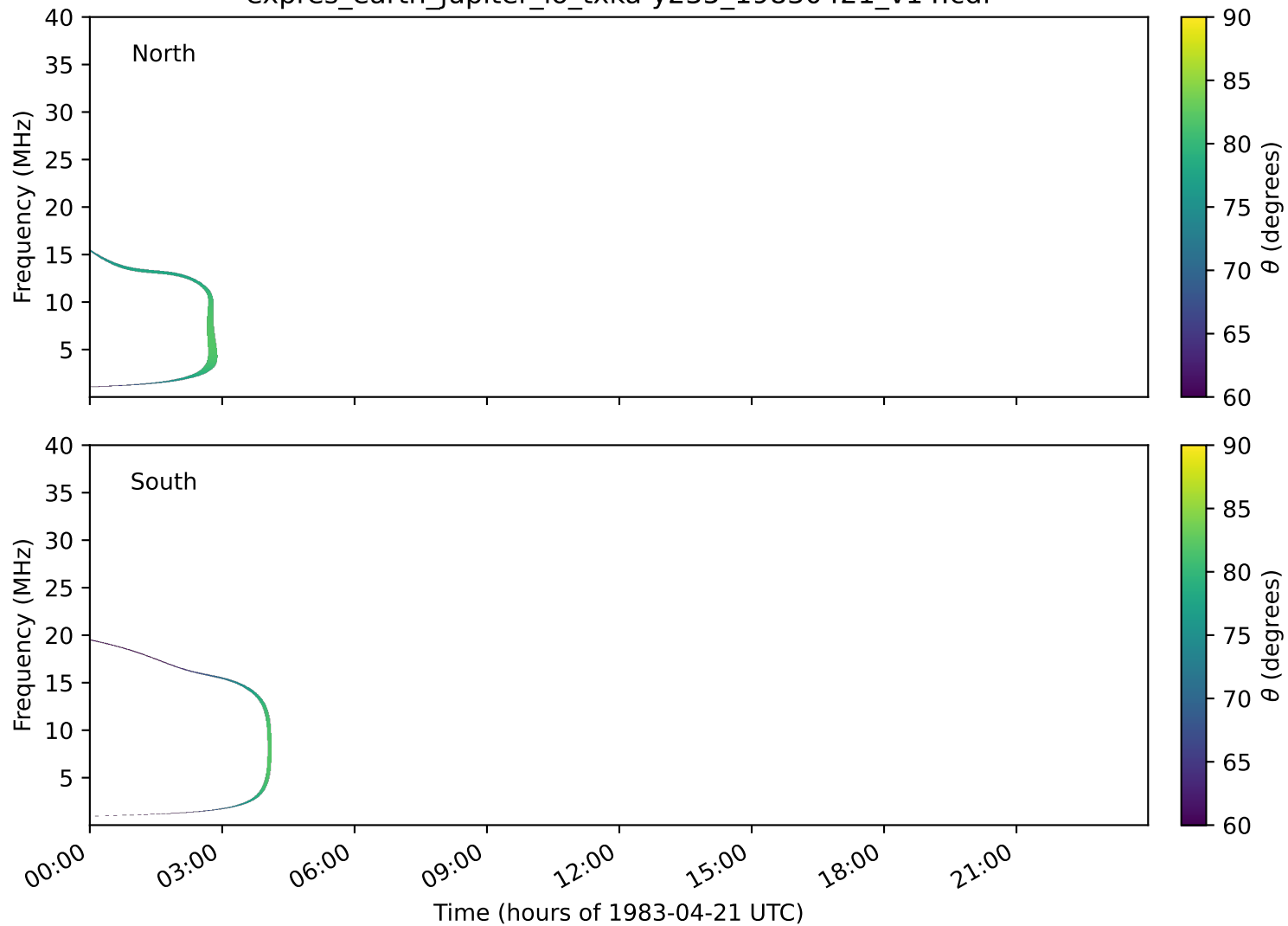
expres_earth_jupiter_io_txka-y235_19830421_v14.cdf
