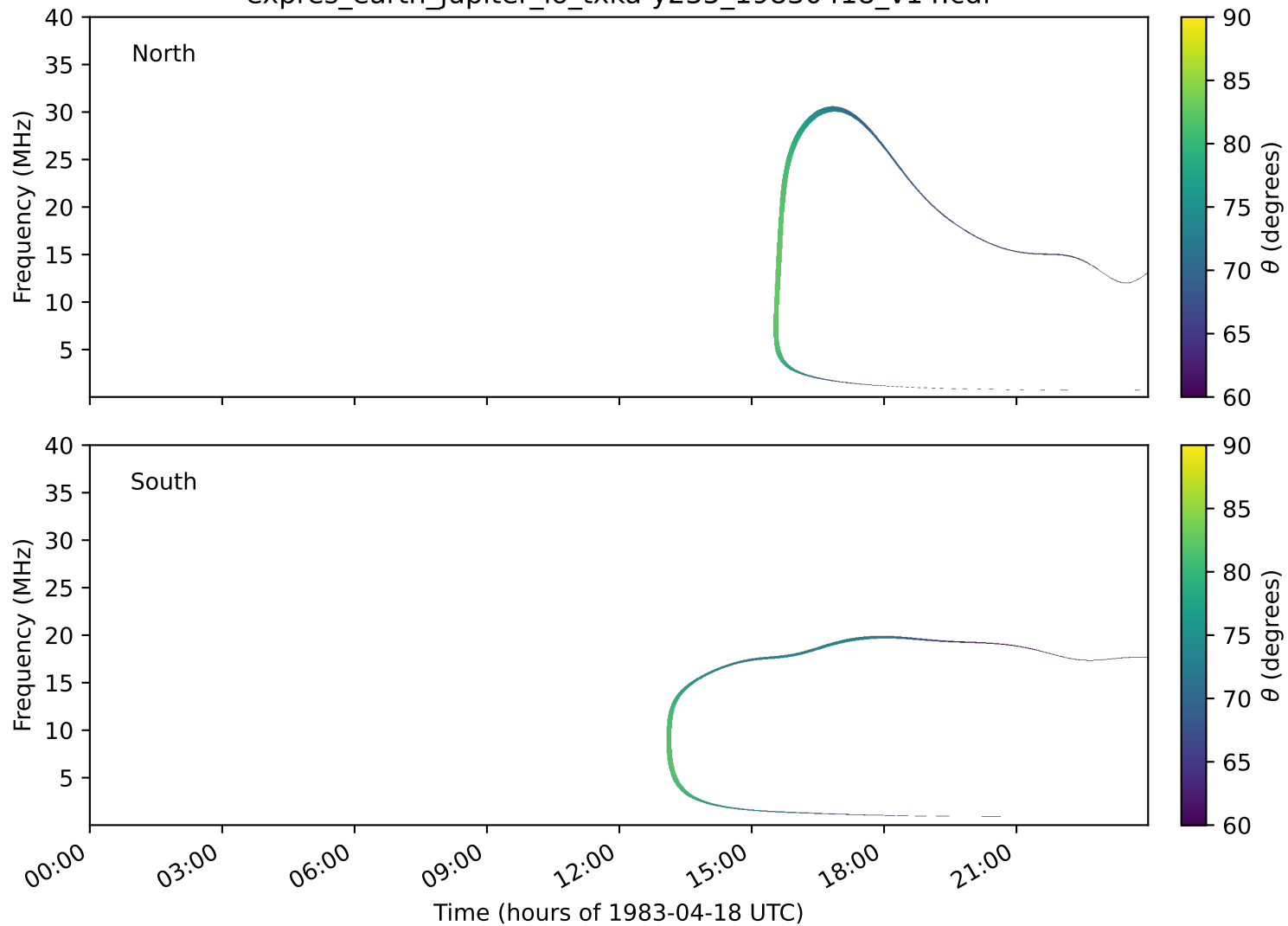
expres_earth_jupiter_io_txka-y235_19830418_v14.cdf
