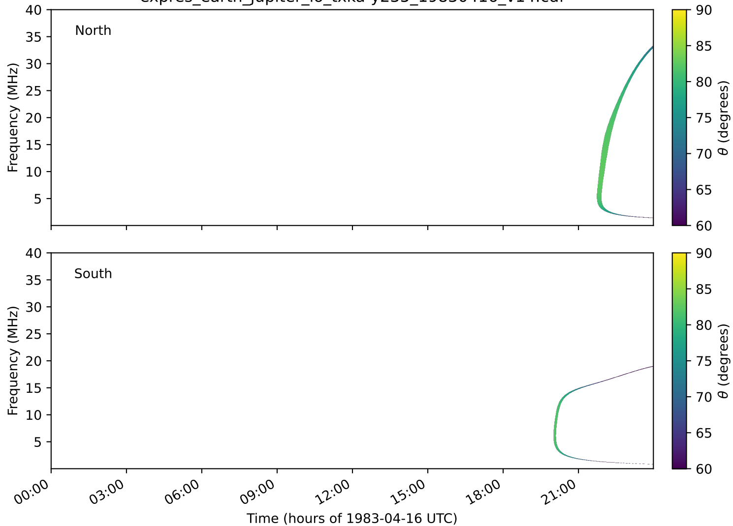
expres_earth_jupiter_io_txka-y235_19830416_v14.cdf
