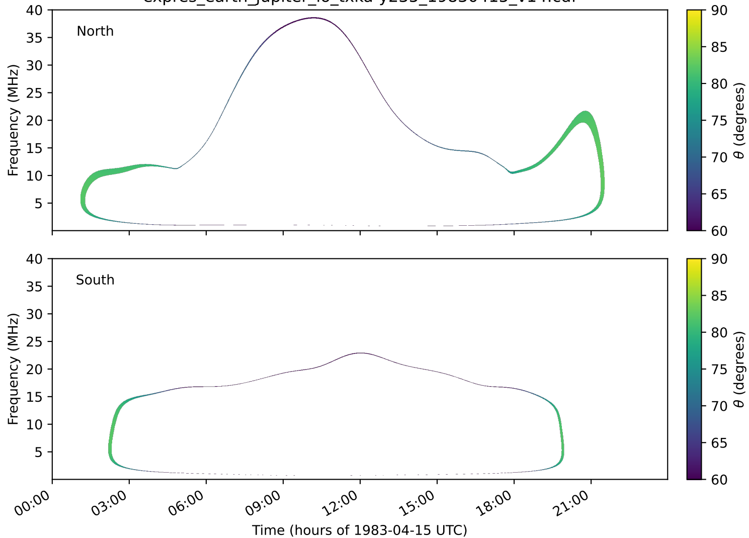
expres_earth_jupiter_io_txka-y235_19830415_v14.cdf
