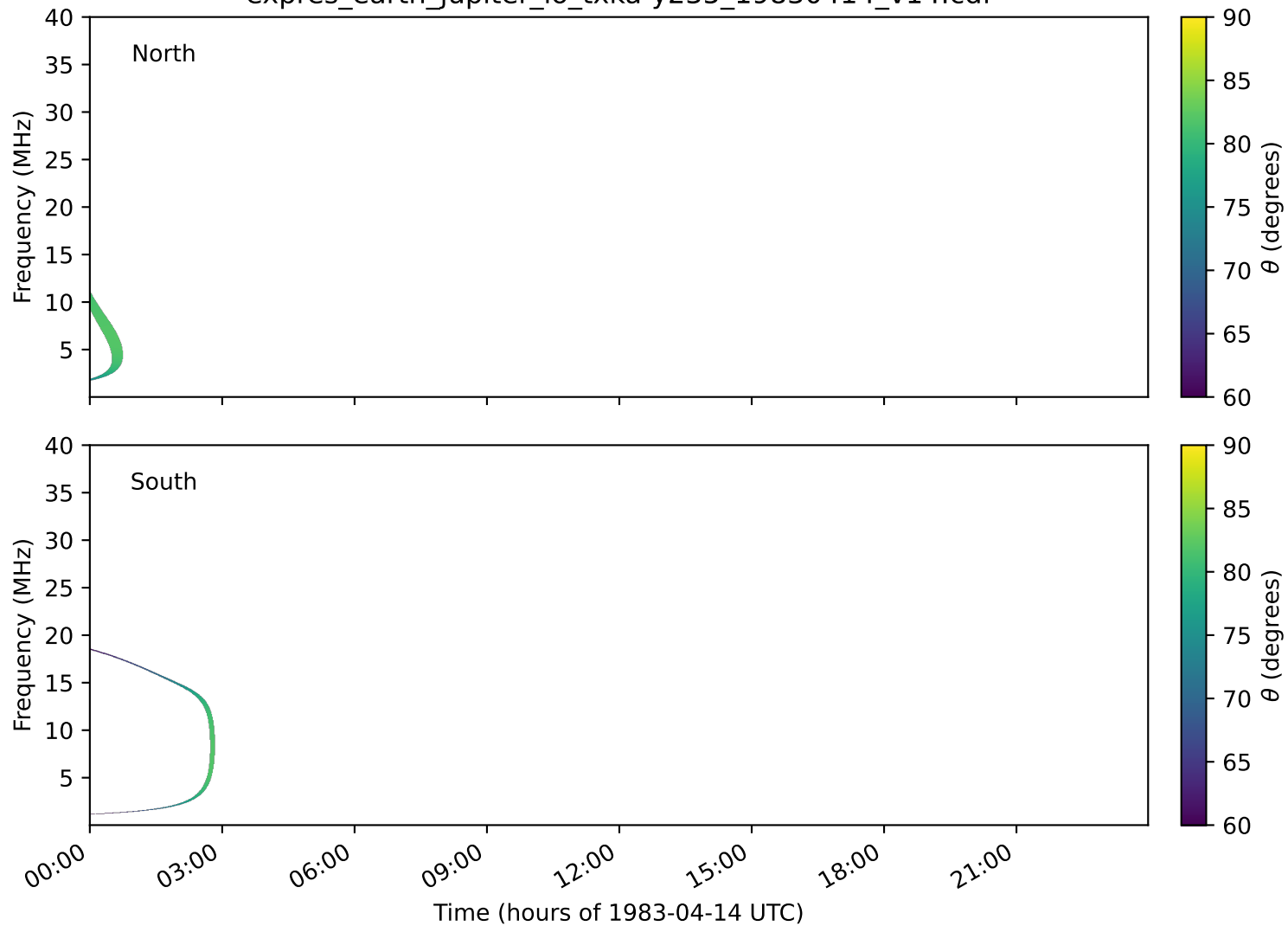
expres_earth_jupiter_io_txka-y235_19830414_v14.cdf
