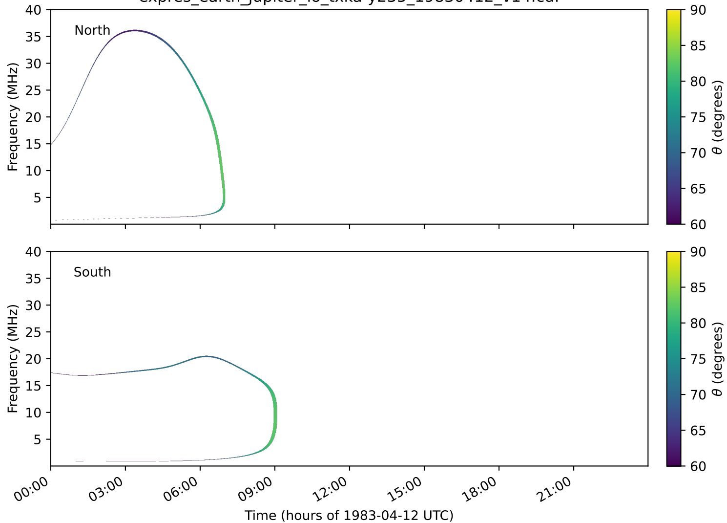
expres_earth_jupiter_io_txka-y235_19830412_v14.cdf
