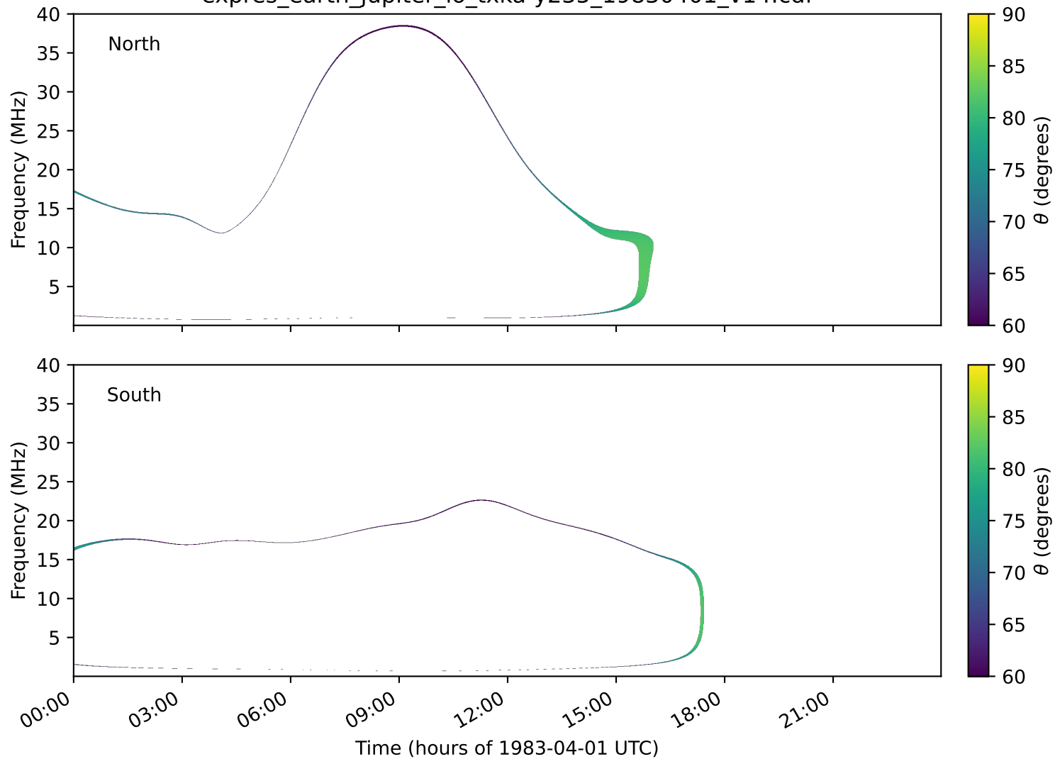
expres_earth_jupiter_io_txka-y235_19830401_v14.cdf
