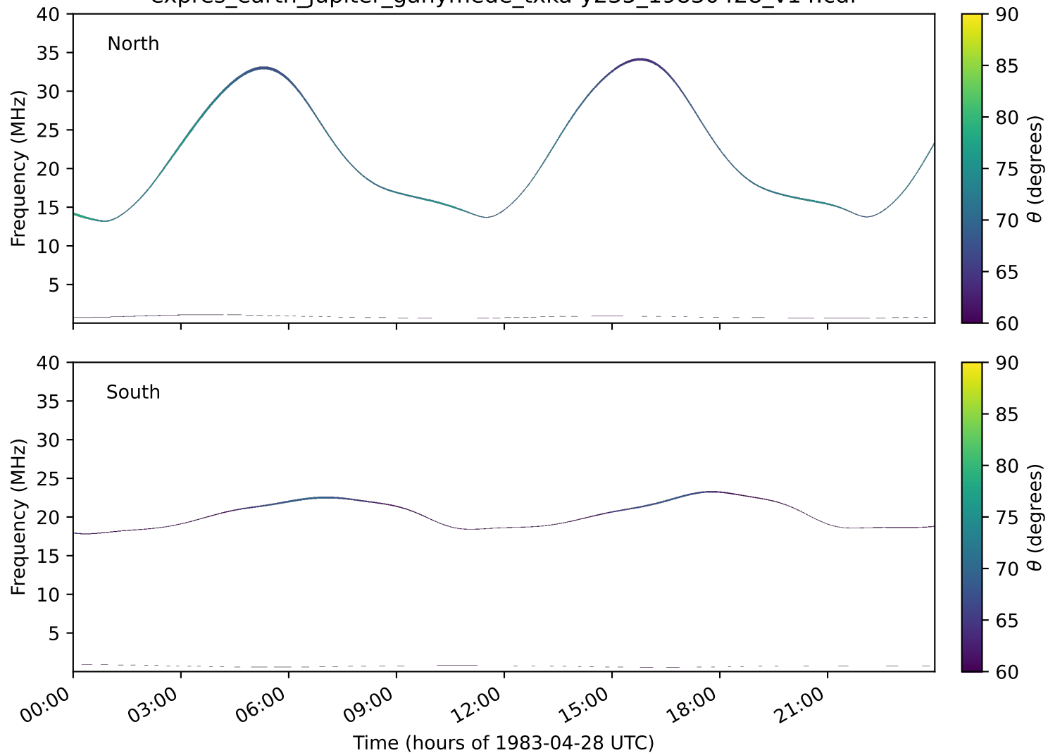
expres_earth_jupiter_ganymede_txka-y235_19830428_v14.cdf
