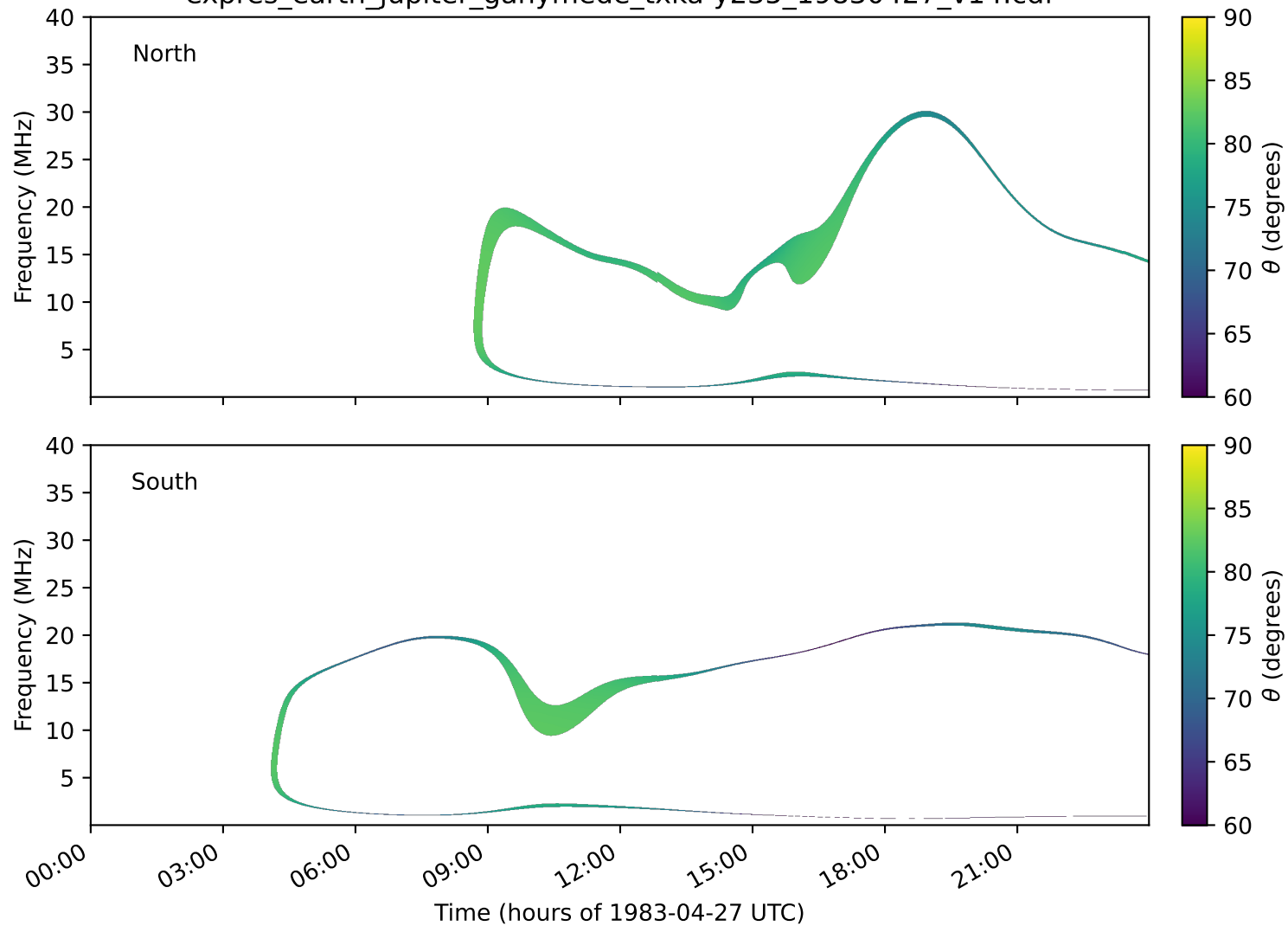
expres_earth_jupiter_ganymede_txka-y235_19830427_v14.cdf
