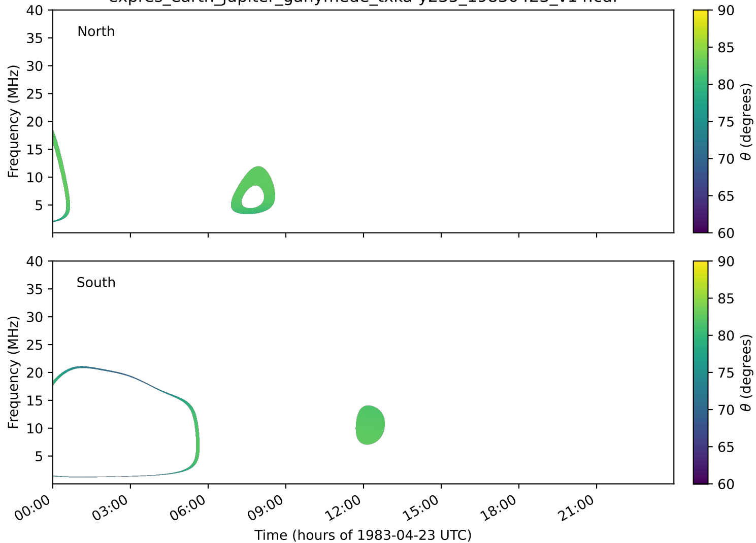
expres_earth_jupiter_ganymede_txka-y235_19830423_v14.cdf
