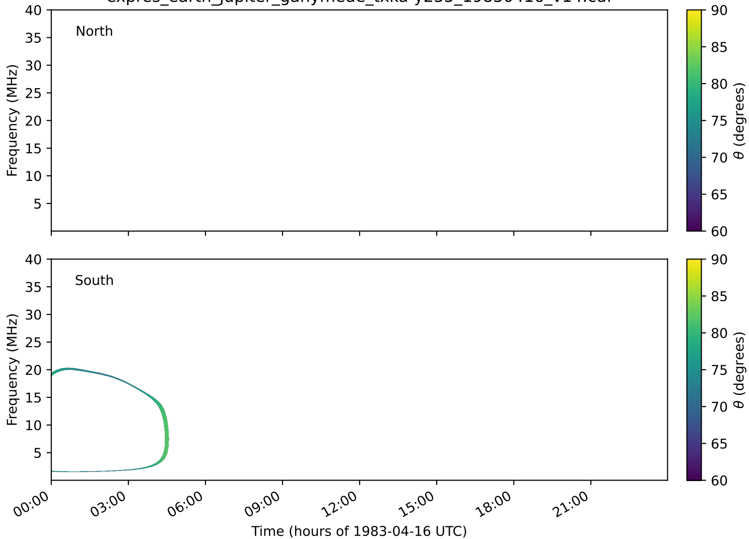
expres_earth_jupiter_ganymede_txka-y235_19830416_v14.cdf
