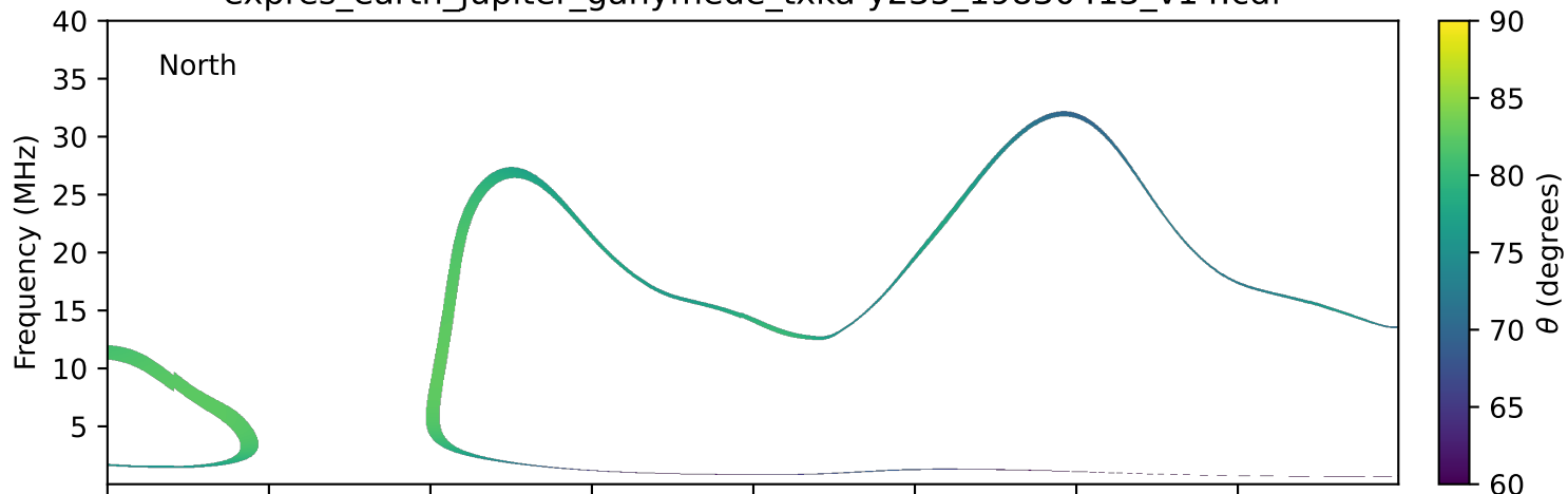
expres_earth_jupiter_ganymede_txka-y235_19830413_v14.cdf
