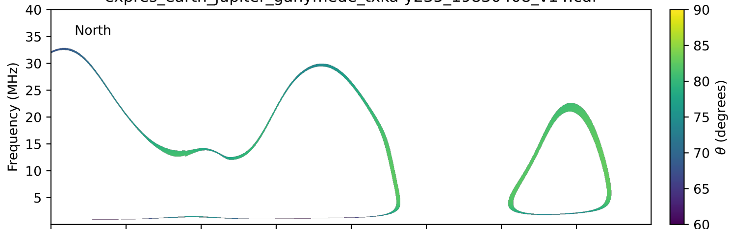
expres_earth_jupiter_ganymede_txka-y235_19830408_v14.cdf
