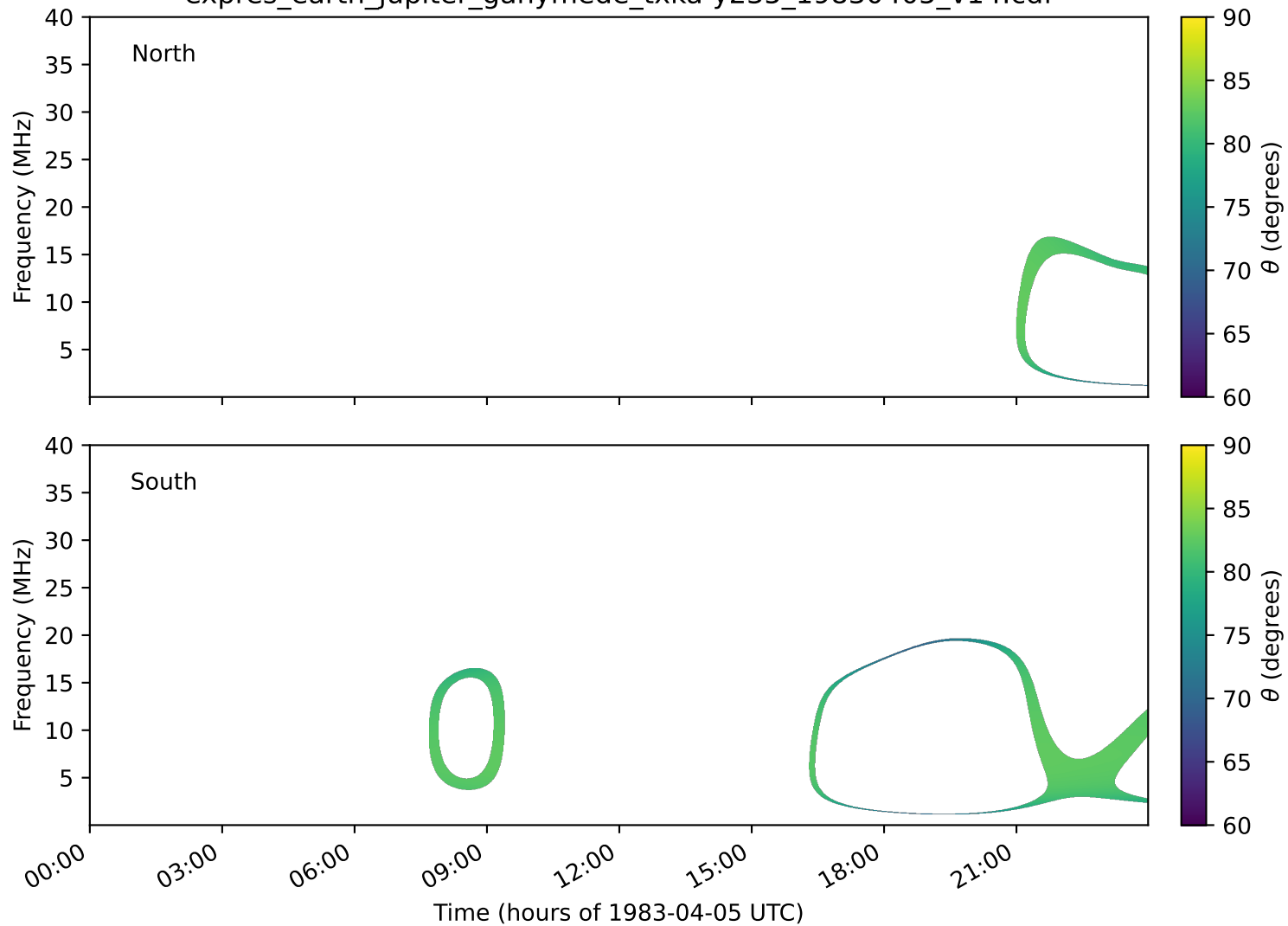
expres_earth_jupiter_ganymede_txka-y235_19830405_v14.cdf
