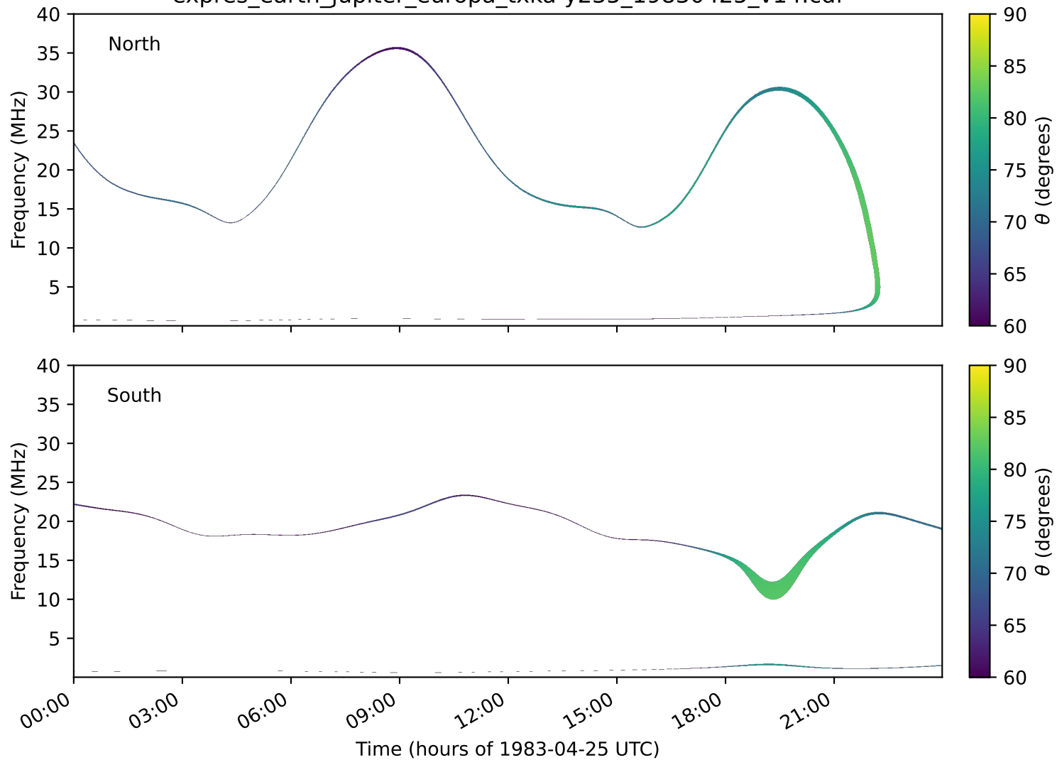
expres_earth_jupiter_europa_txka-y235_19830425_v14.cdf
