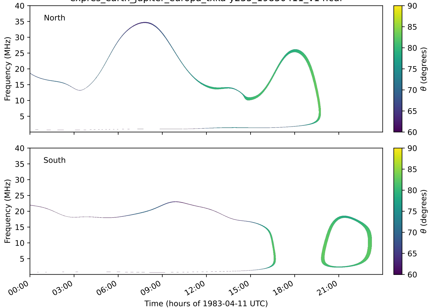
expres_earth_jupiter_europa_txka-y235_19830411_v14.cdf
