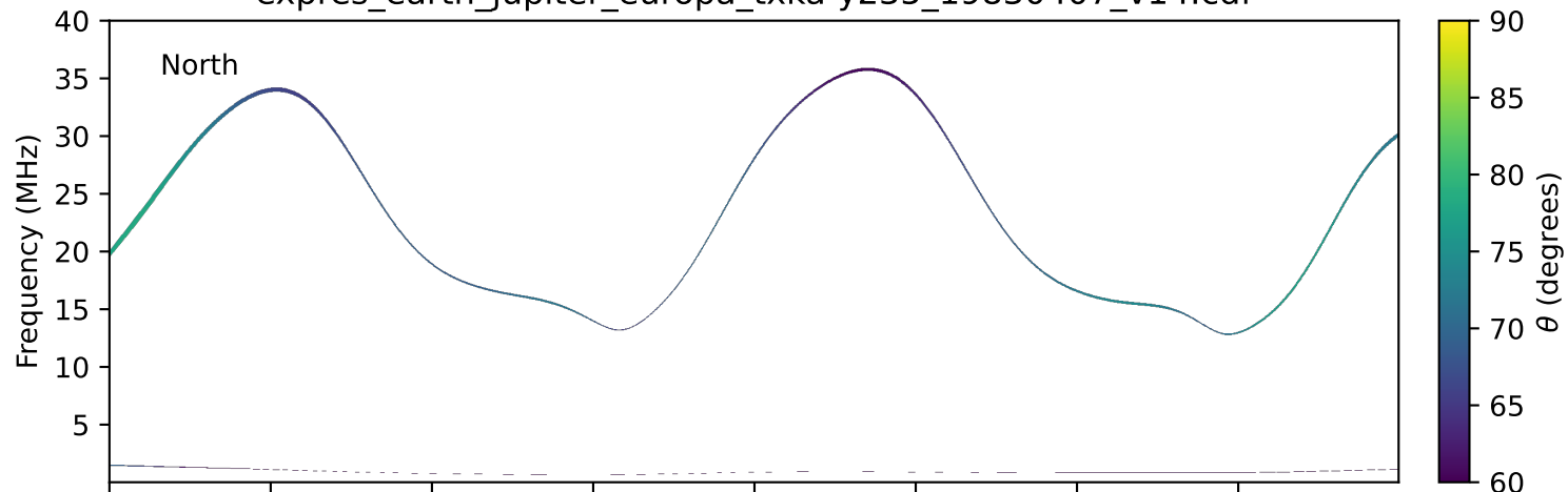
expres_earth_jupiter_europa_txka-y235_19830407_v14.cdf
