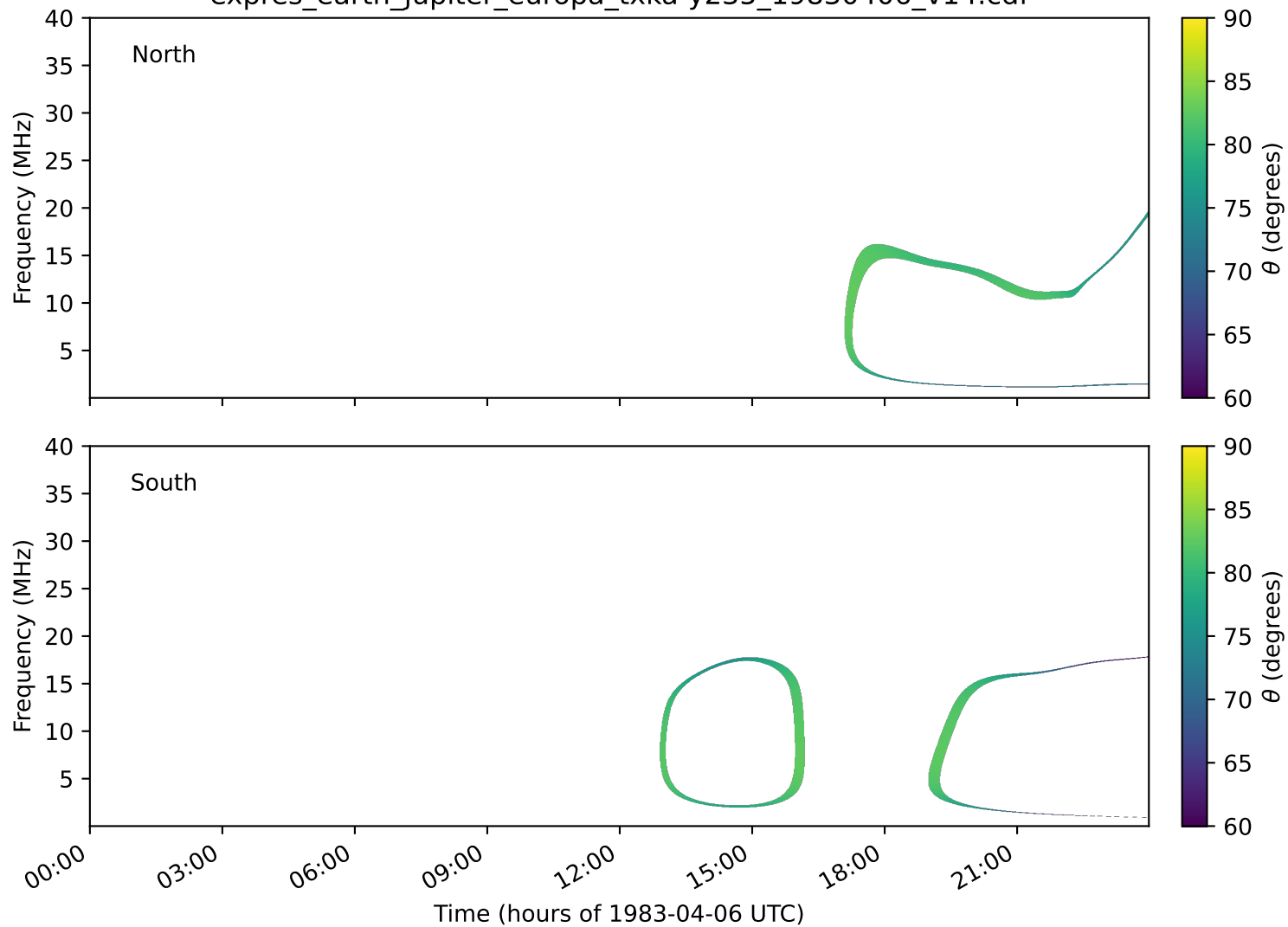
expres_earth_jupiter_europa_txka-y235_19830406_v14.cdf
