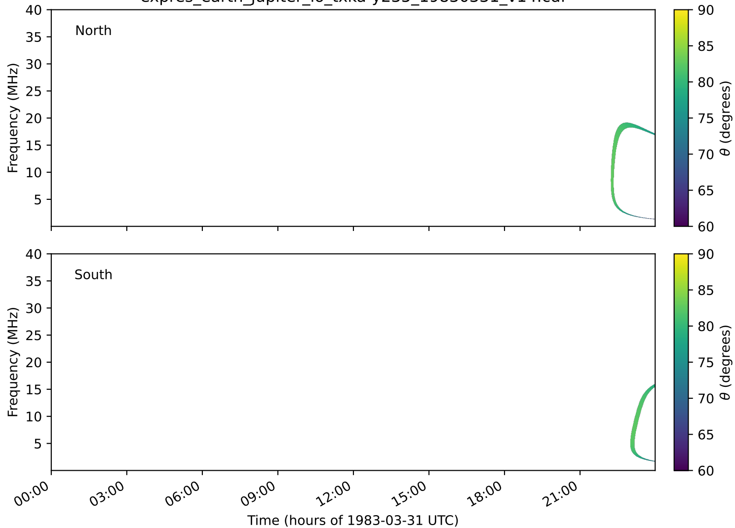
expres_earth_jupiter_io_txka-y235_19830331_v14.cdf
