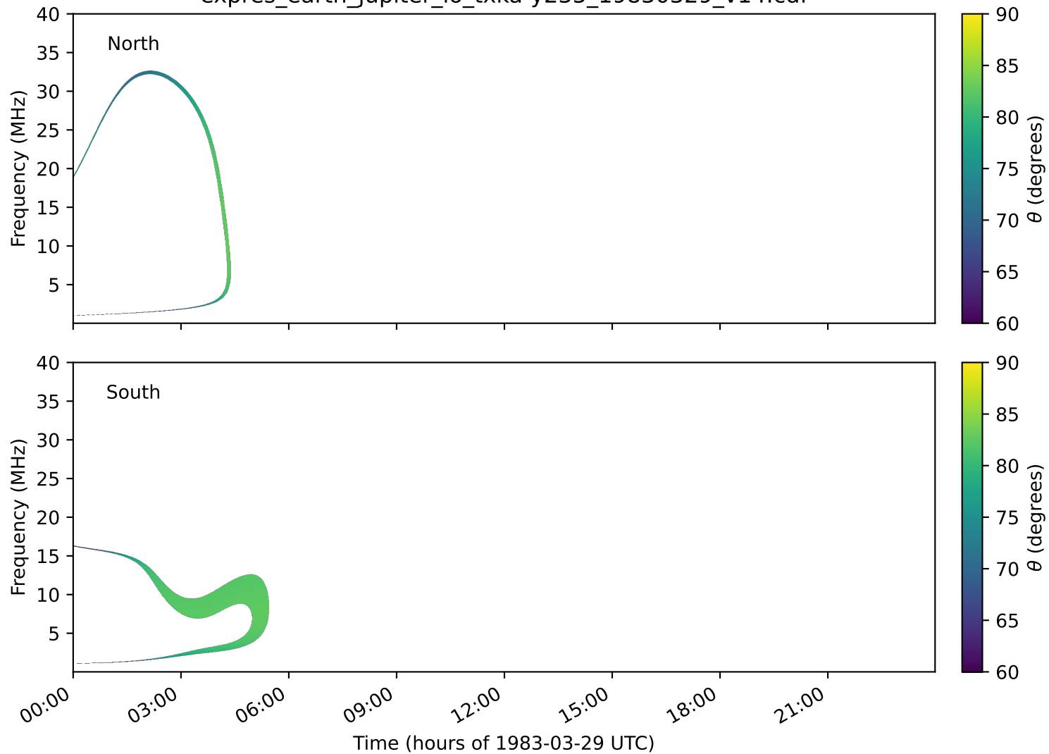
expres_earth_jupiter_io_txka-y235_19830329_v14.cdf
