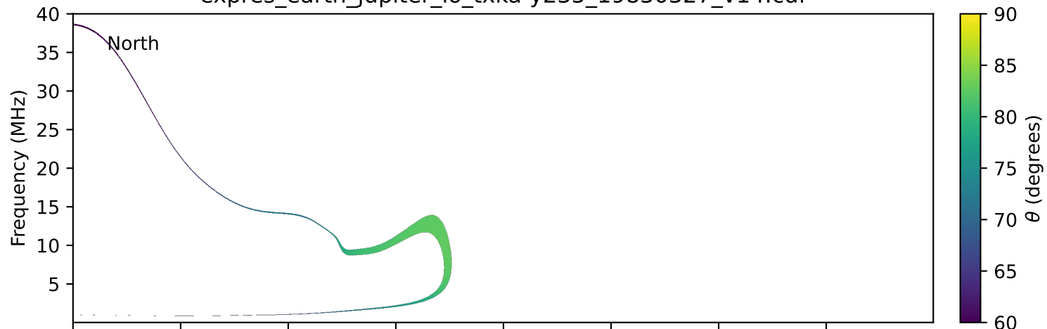
expres_earth_jupiter_io_txka-y235_19830327_v14.cdf
