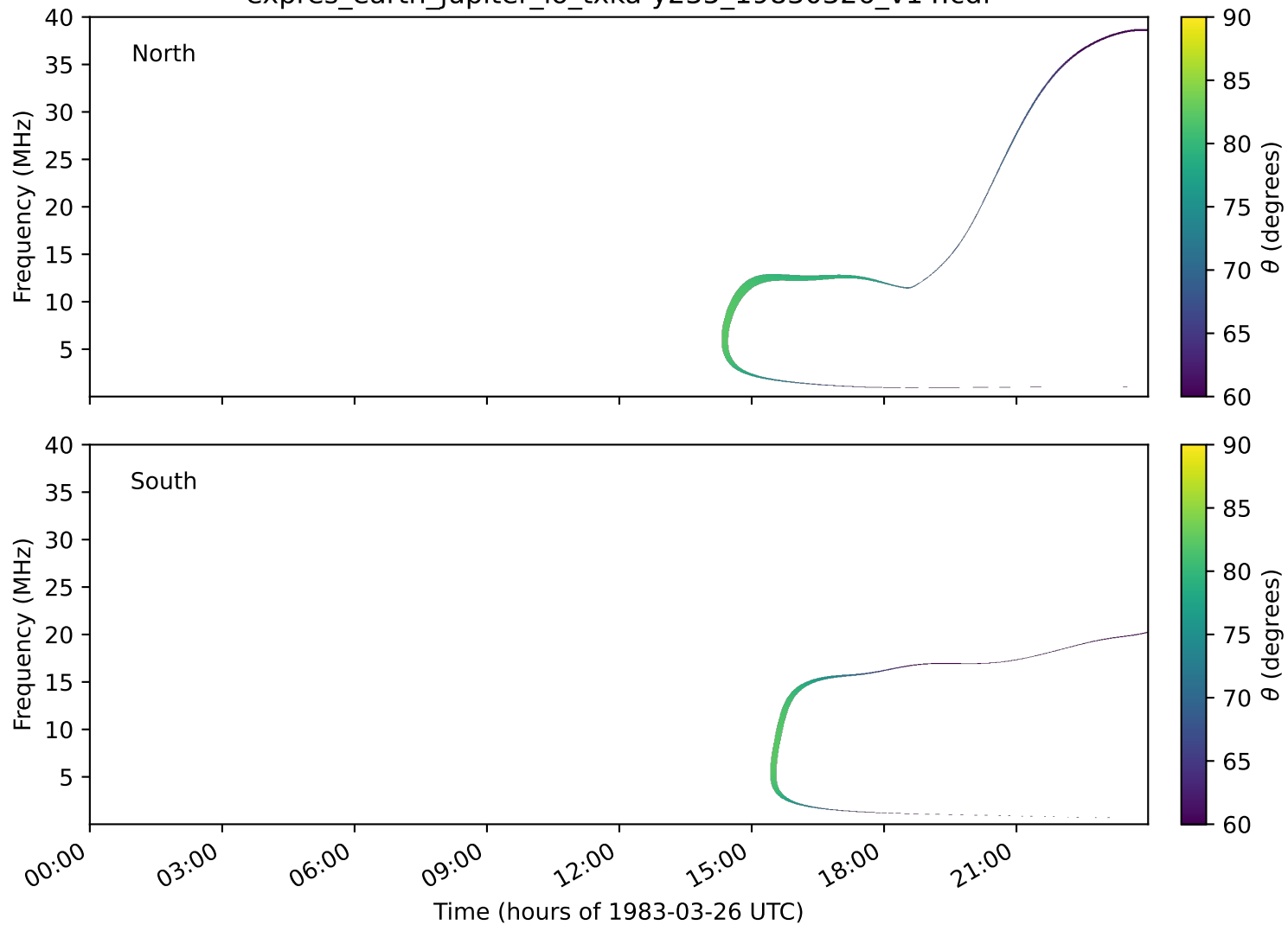
expres_earth_jupiter_io_txka-y235_19830326_v14.cdf
