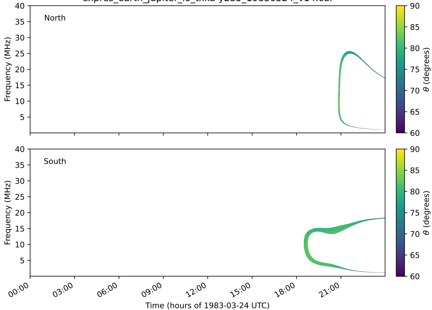
expres_earth_jupiter_io_txka-y235_19830324_v14.cdf
