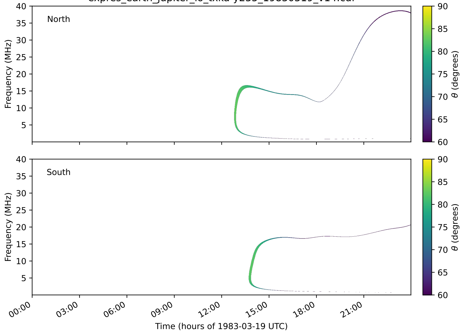
expres_earth_jupiter_io_txka-y235_19830319_v14.cdf
