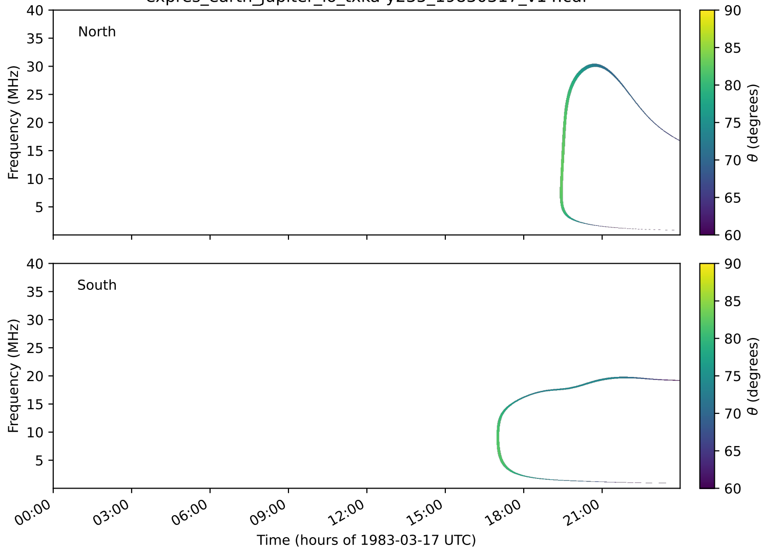
expres_earth_jupiter_io_txka-y235_19830317_v14.cdf
