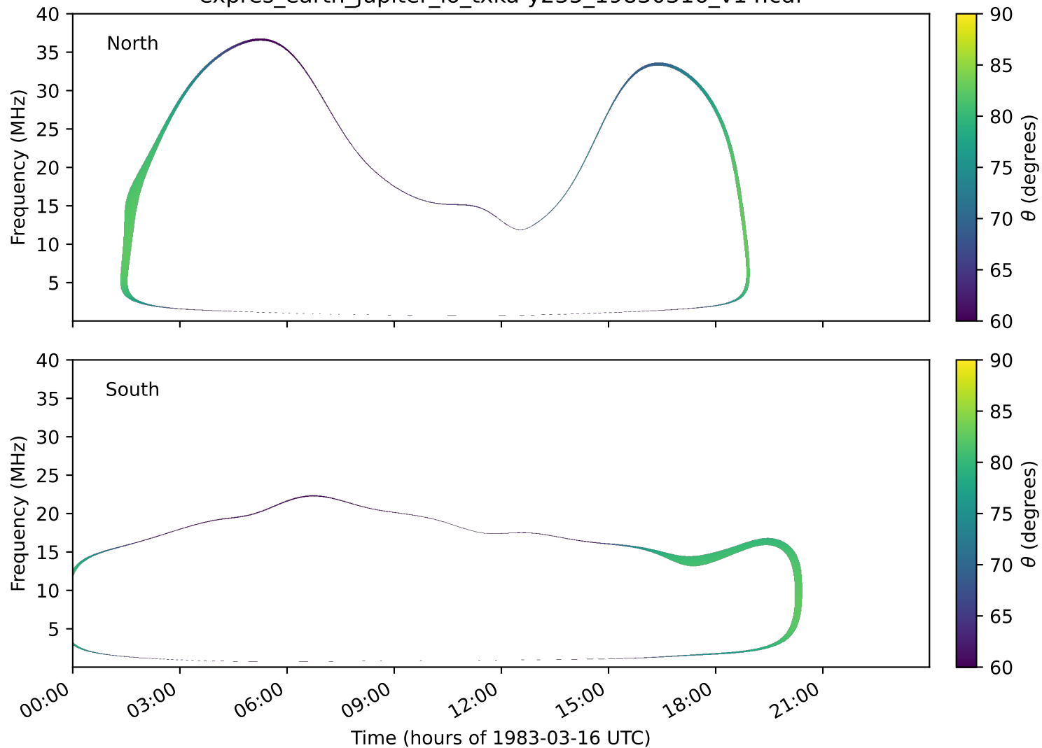
expres_earth_jupiter_io_txka-y235_19830316_v14.cdf
