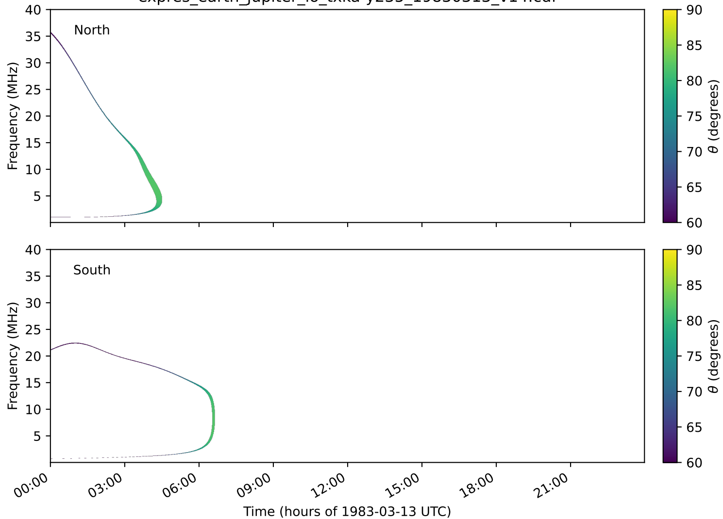
expres_earth_jupiter_io_txka-y235_19830313_v14.cdf
