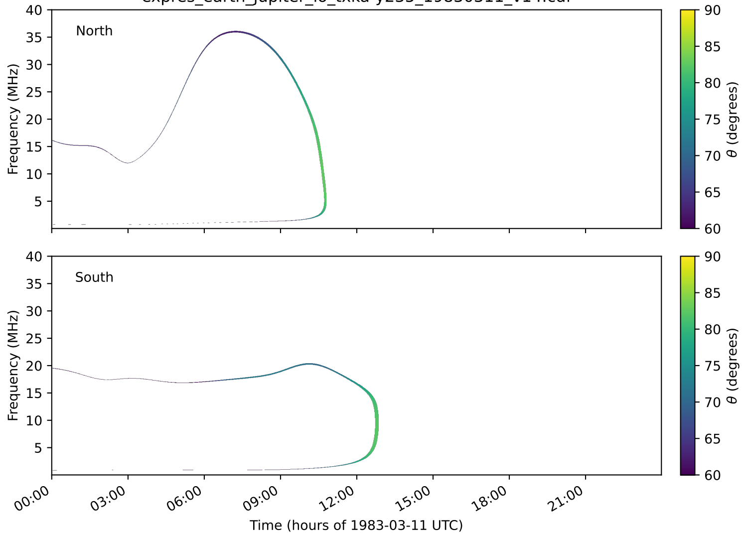
expres_earth_jupiter_io_txka-y235_19830311_v14.cdf
