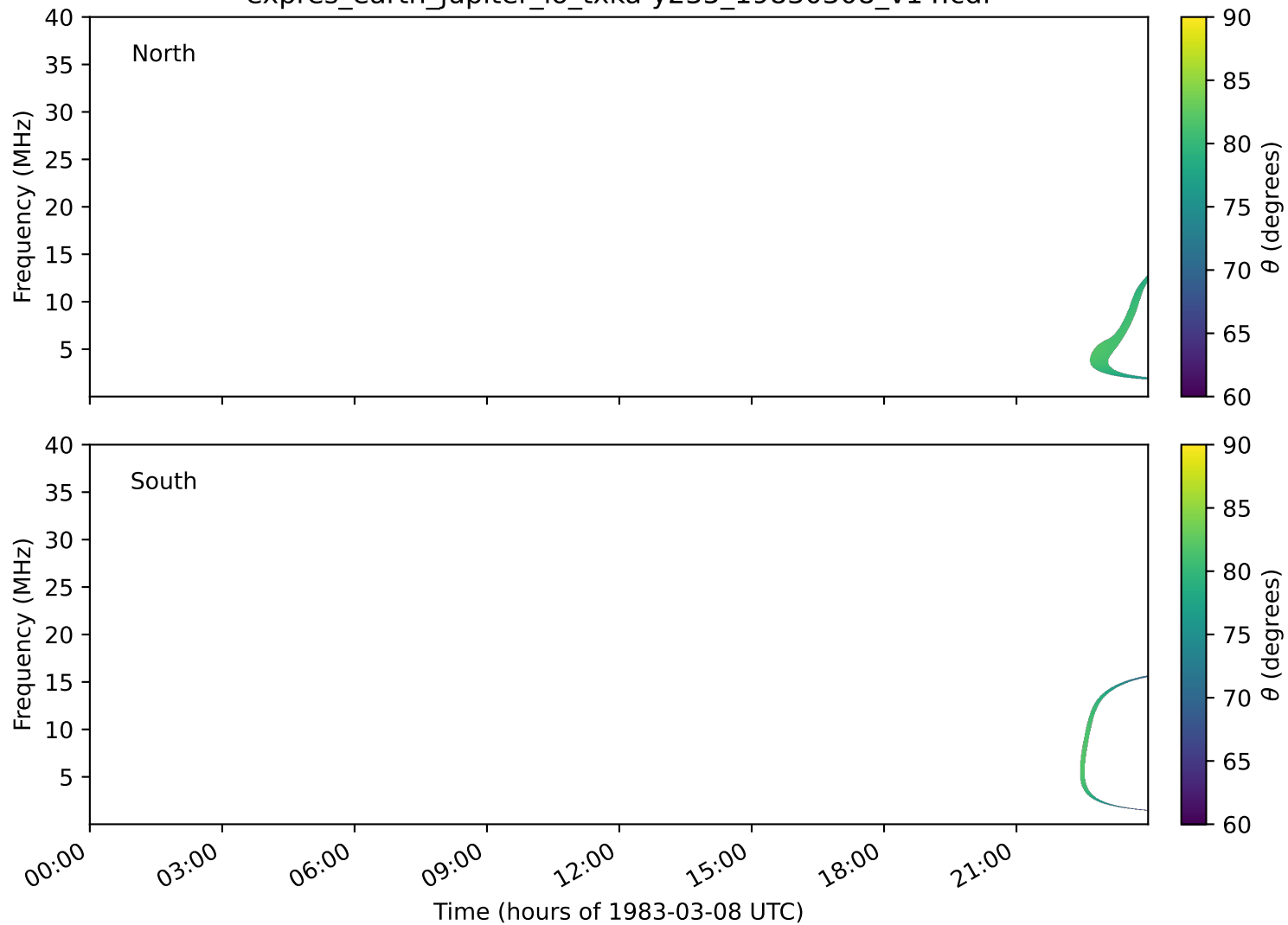
expres_earth_jupiter_io_txka-y235_19830308_v14.cdf
