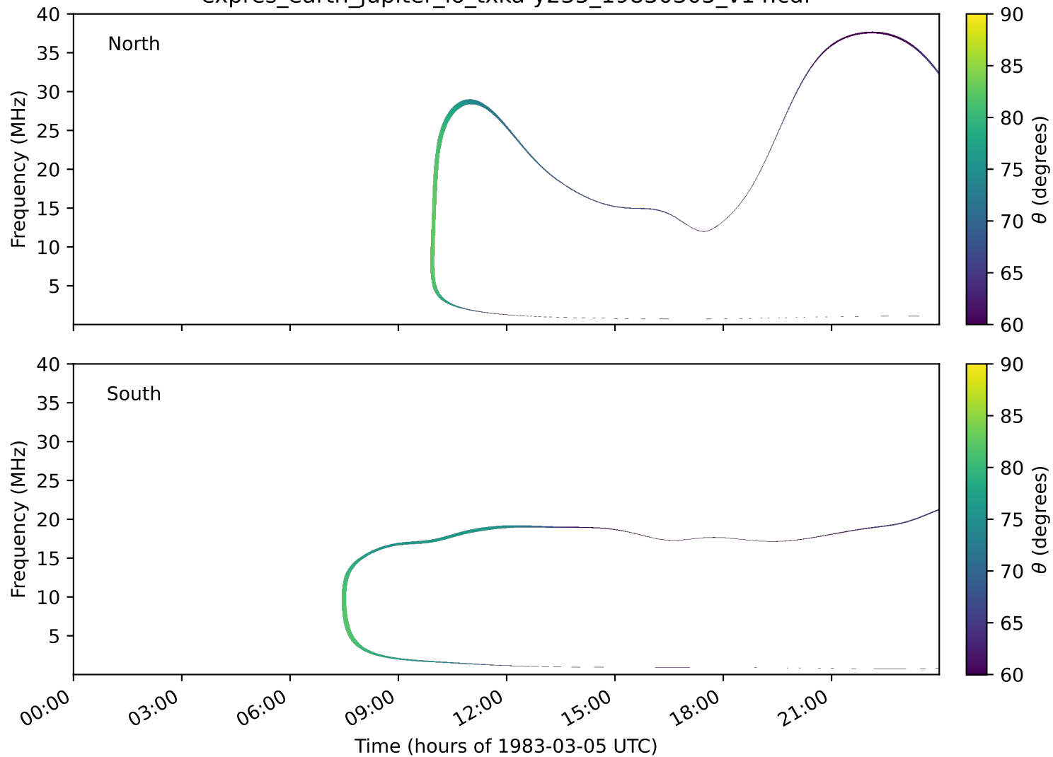
expres_earth_jupiter_io_txka-y235_19830305_v14.cdf
