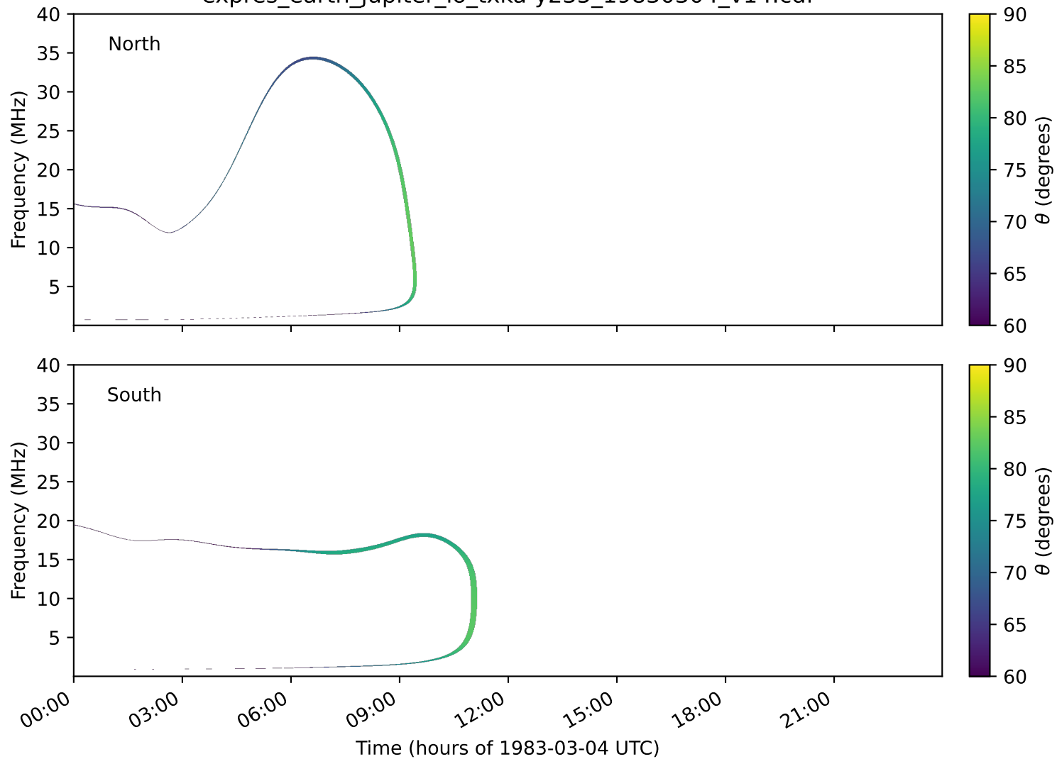
expres_earth_jupiter_io_txka-y235_19830304_v14.cdf
