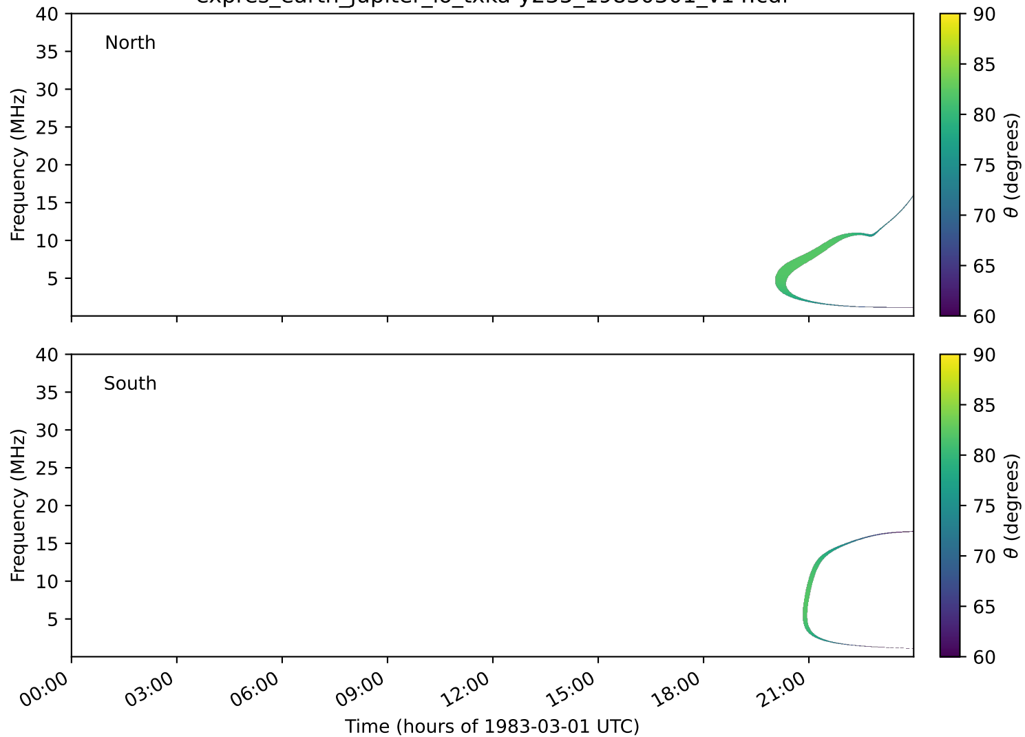
expres_earth_jupiter_io_txka-y235_19830301_v14.cdf
