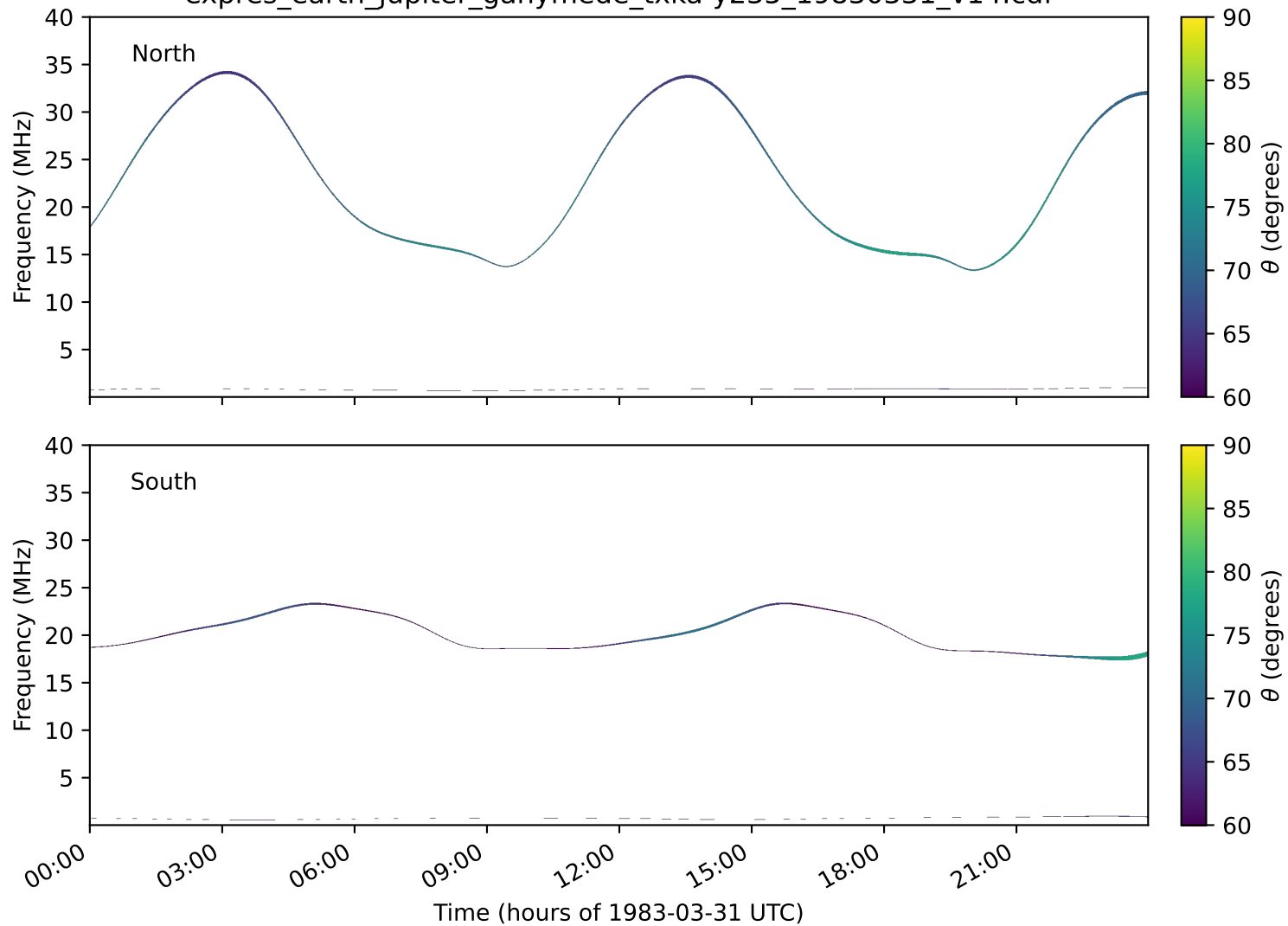
expres_earth_jupiter_ganymede_txka-y235_19830331_v14.cdf
