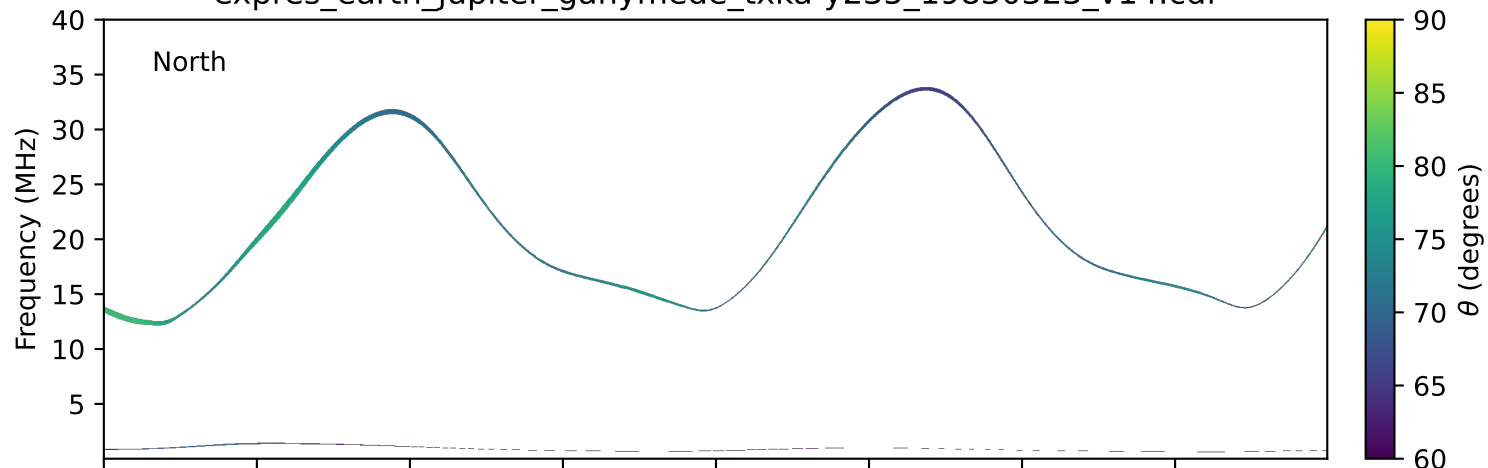
expres_earth_jupiter_ganymede_txka-y235_19830323_v14.cdf
