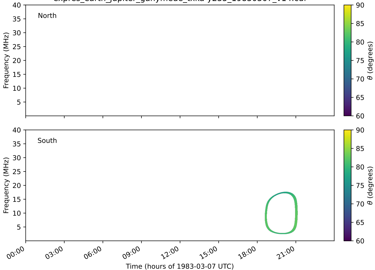
expres_earth_jupiter_ganymede_txka-y235_19830307_v14.cdf
