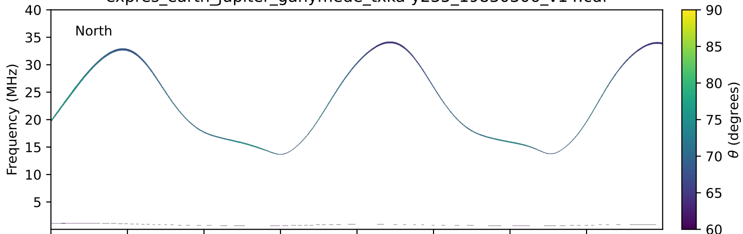
expres_earth_jupiter_ganymede_txka-y235_19830306_v14.cdf
