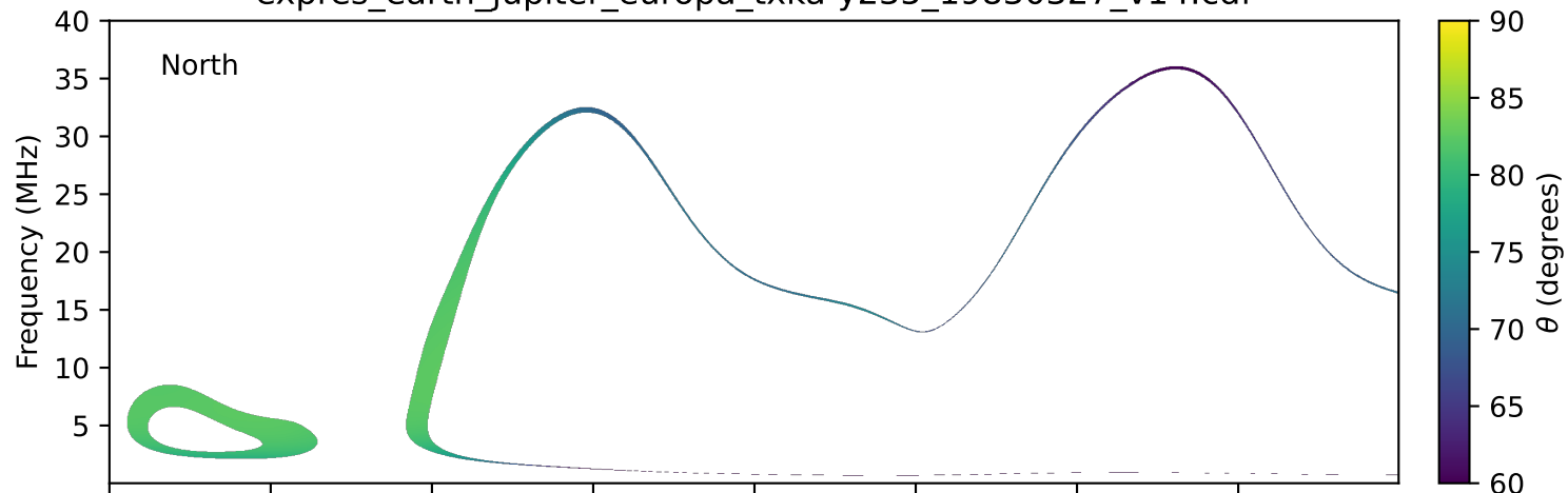
expres_earth_jupiter_europa_txka-y235_19830327_v14.cdf
