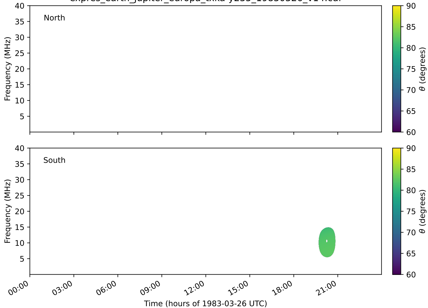
expres_earth_jupiter_europa_txka-y235_19830326_v14.cdf
