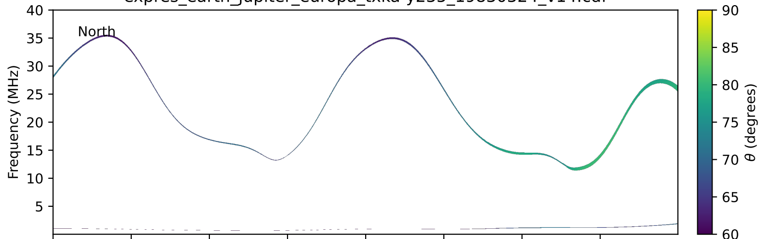
expres_earth_jupiter_europa_txka-y235_19830324_v14.cdf
