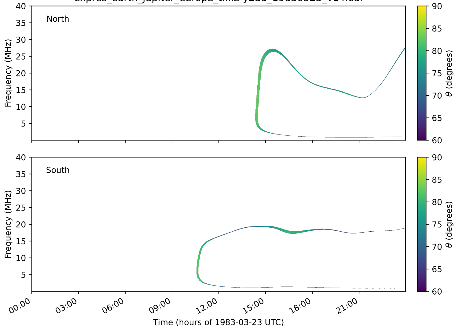
expres_earth_jupiter_europa_txka-y235_19830323_v14.cdf
