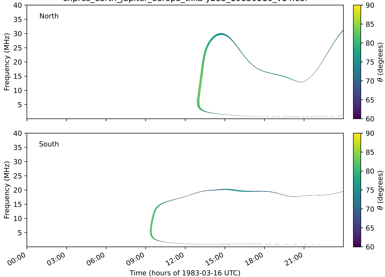
expres_earth_jupiter_europa_txka-y235_19830316_v14.cdf
