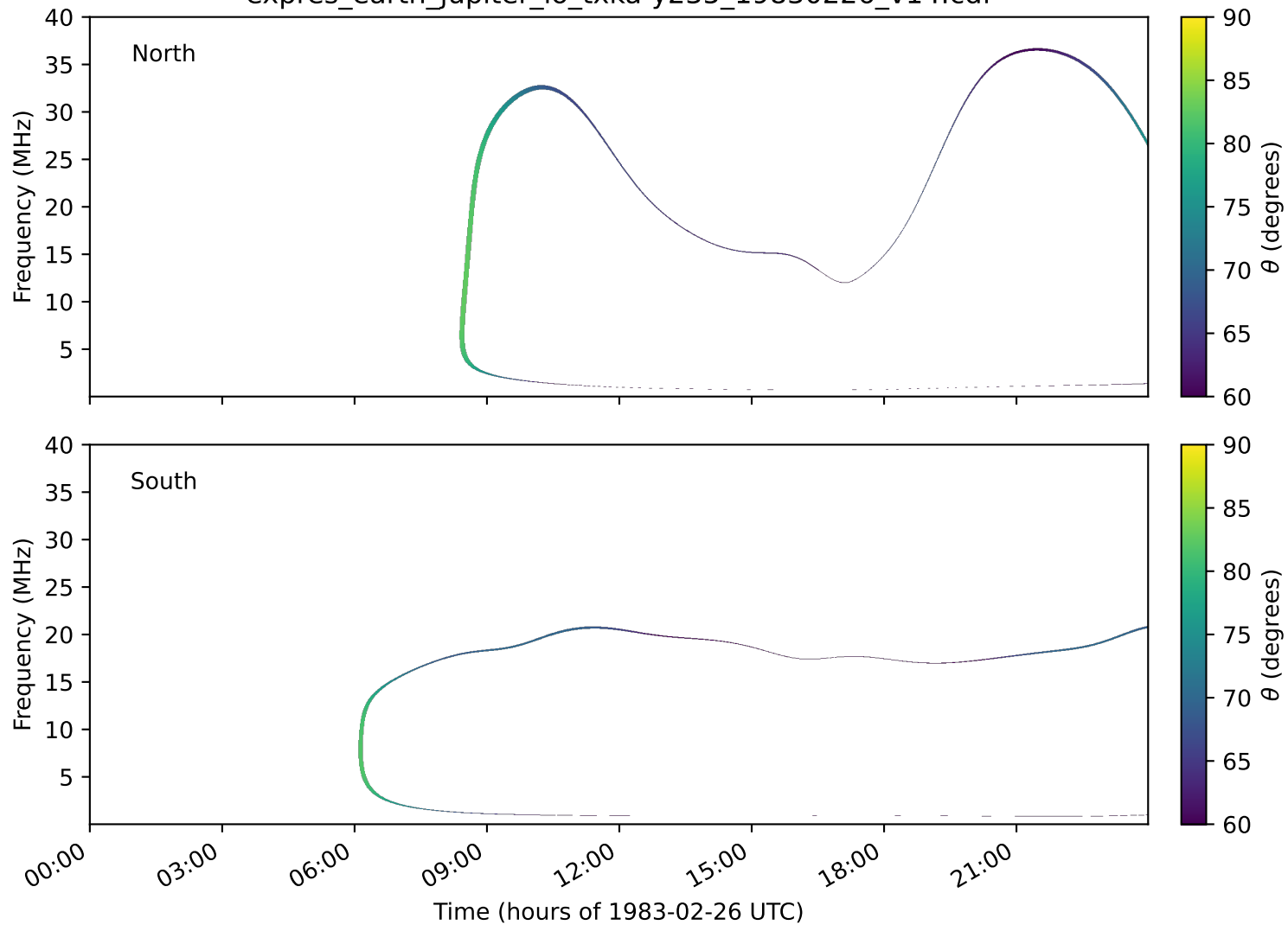
expres_earth_jupiter_io_txka-y235_19830226_v14.cdf
