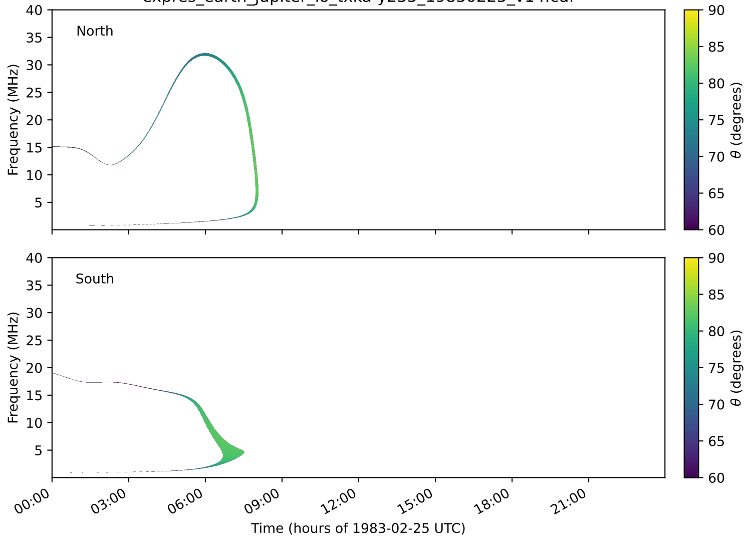
expres_earth_jupiter_io_txka-y235_19830225_v14.cdf
