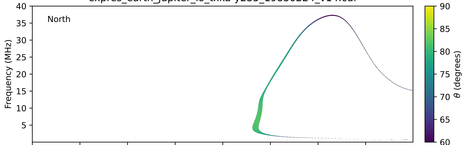
expres_earth_jupiter_io_txka-y235_19830224_v14.cdf
